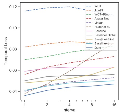
Figure 6: Quantitative evaluation of temporal consistency. For the proposed method, Baseline denotes the proposed image style transfer network, Blind denotes using Blind (Lai et al. 2018) for post-processing, \mathcal{L}_t denotes training with temporal loss, and Global denotes using global feature sharing. Our models yields the lowest temporal loss for all temporal length.
