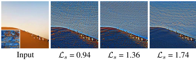
Figure 11: Results of models with different style loss. We choose three models with similar temporal loss (0.0478 ~ 0.0481) but various style loss \mathcal{L}_s . Models with higher style loss fail to well reconstruct the wooden texture.
