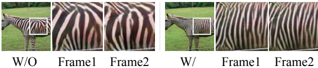
Figure 12: With the proposed temporal regularization, the temporal consistency of CycleGAN improves.
