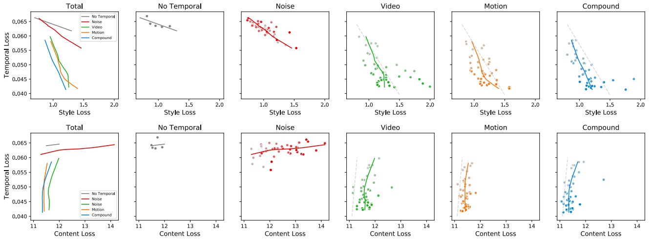
Figure 10: Performance of temporal consistency and stylization. Each data point represents an individual experiment. The strength of regularization is represented by different colors. A deeper color indicates a higher temporal loss weight. For the convenience of comparison, we additionally draw some light gray dotted lines.
