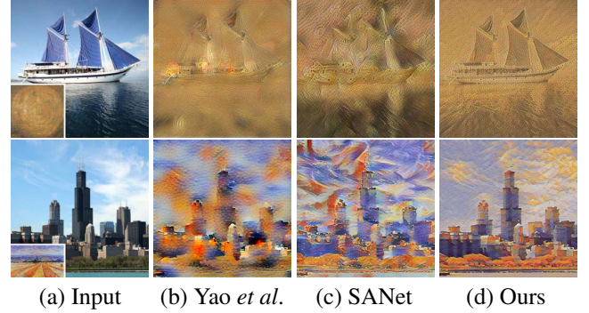
Figure 5: Comparison with other style transfer modules.
