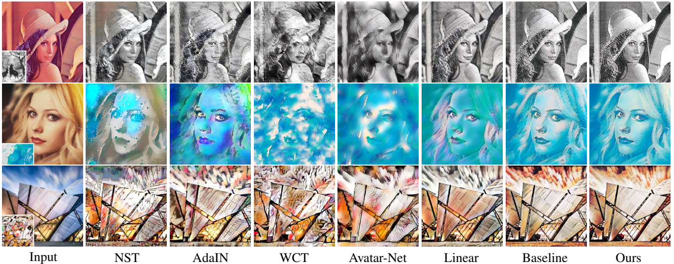
Figure 8: Comparison with state-of-the-art methods on image style transfer.
